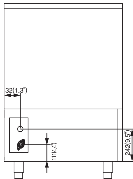
BACK
